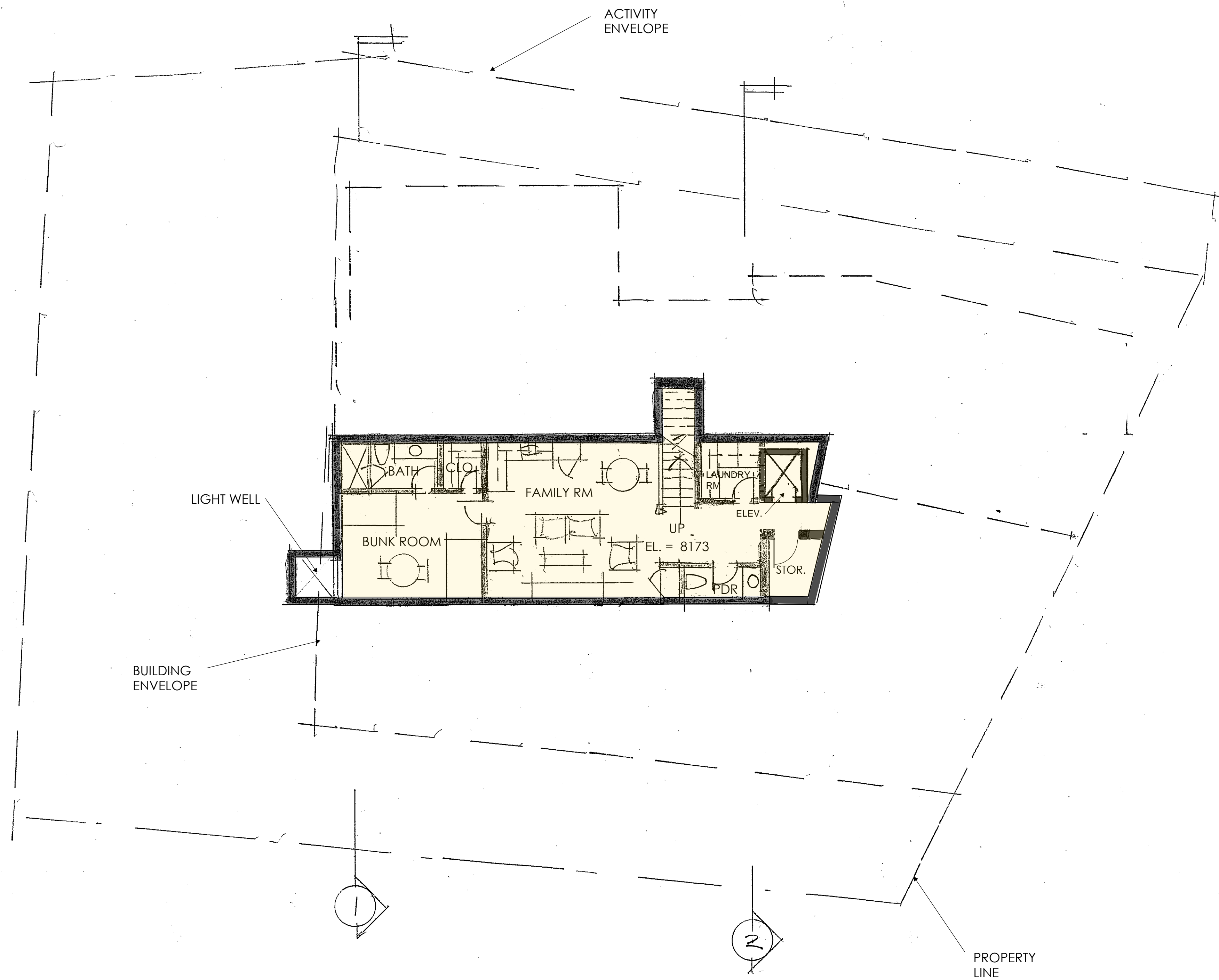
BASEMENT PLAN
